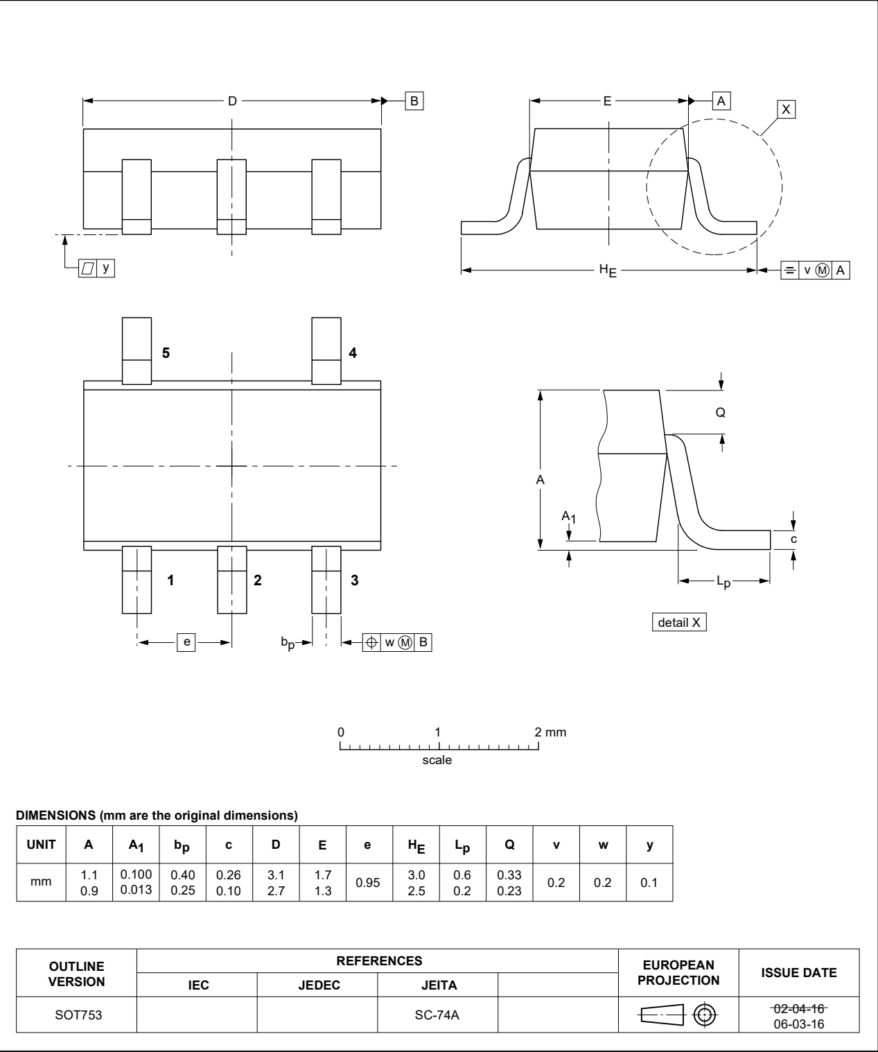
Fig. 22. Package outline SOT753 (SC-74A)
