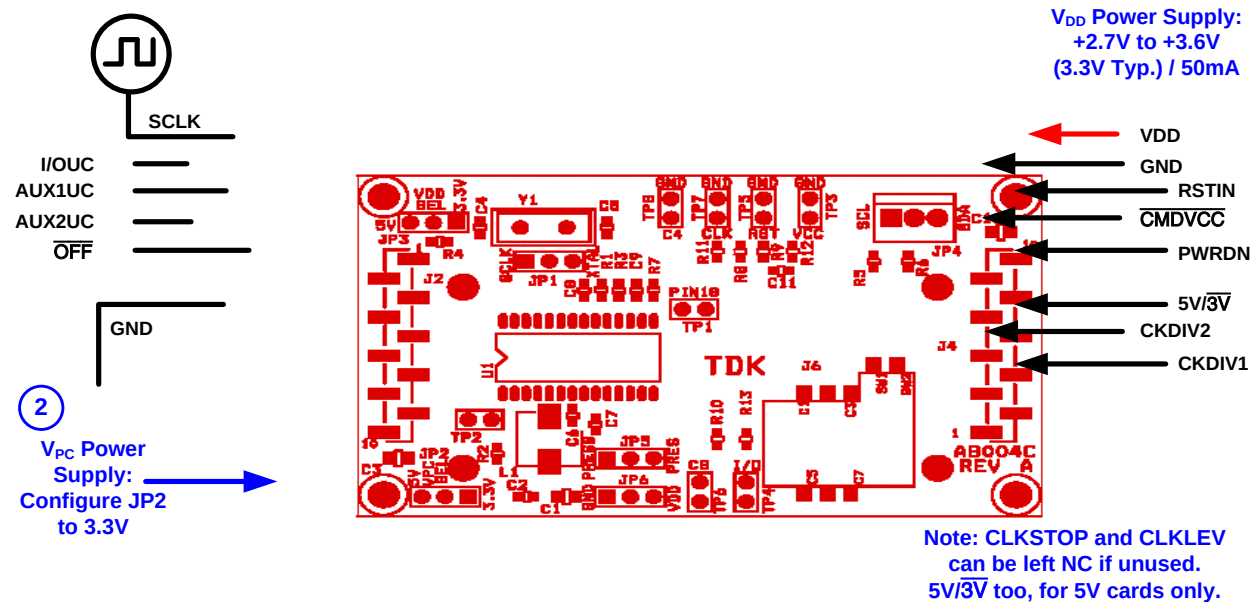
Figure 2: 73S8024C Demo Board Basic Connections
