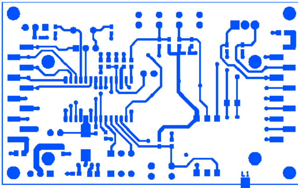
Figure 8: 73S8024C Demo Board Top Signal Layer
