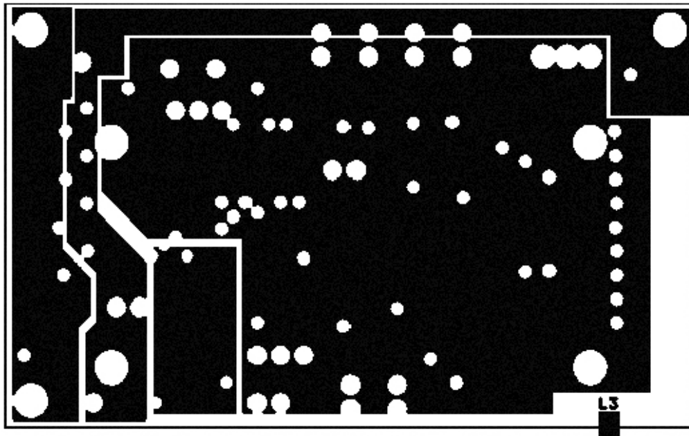
Figure 10: 73S8024C Middle Layer 2, Supply Plane
