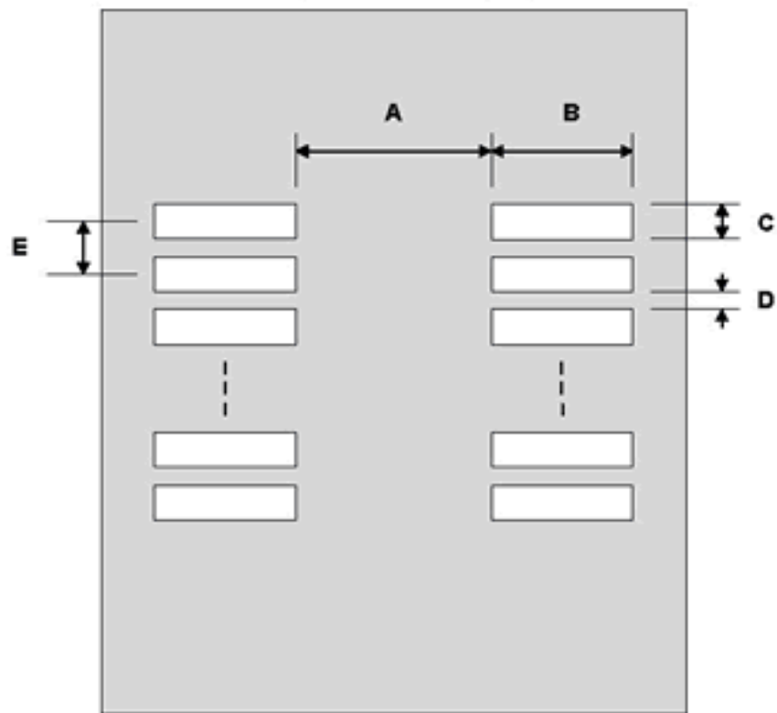
Top View (SMT Footprint)
