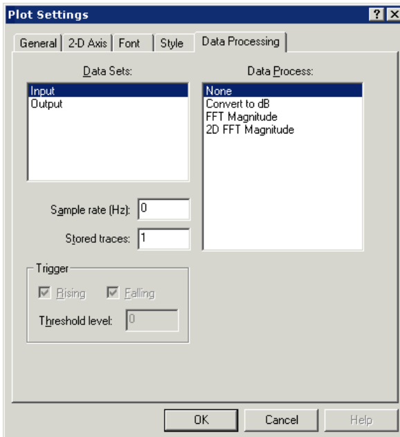
Figure 2-29. Data Processing Page
