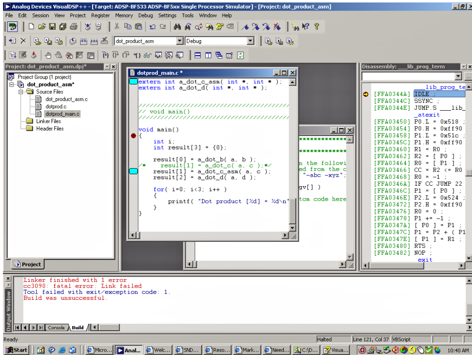
Figure 2-16. Modifying dotprod_main.c to Call a_dot_c_asm
