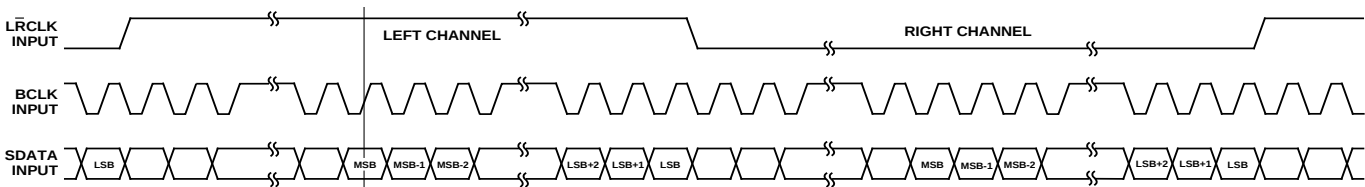
Figure 2. Right-Justified Mode
