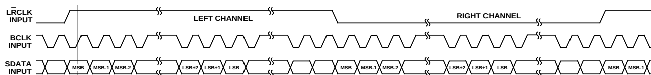
Figure 4. Left-Justified Mode
