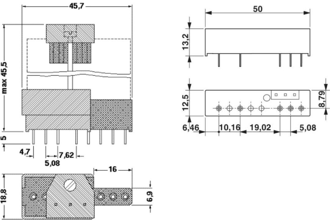
Dimensioned drawing
