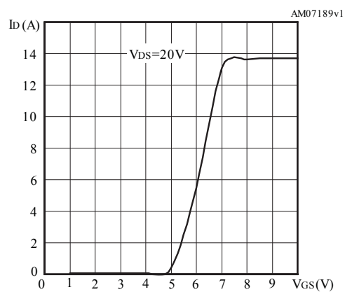
Figure 6. Transfer characteristics
