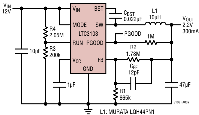
12V to 2.2V/300mA Regulator with 9V Accurate UVLO
