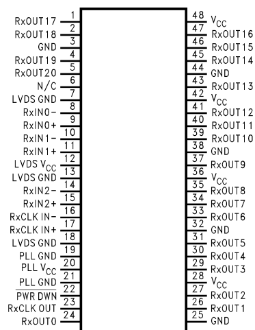
Figure 24. DS90CF364
