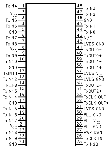
Figure 23. DS90C363
