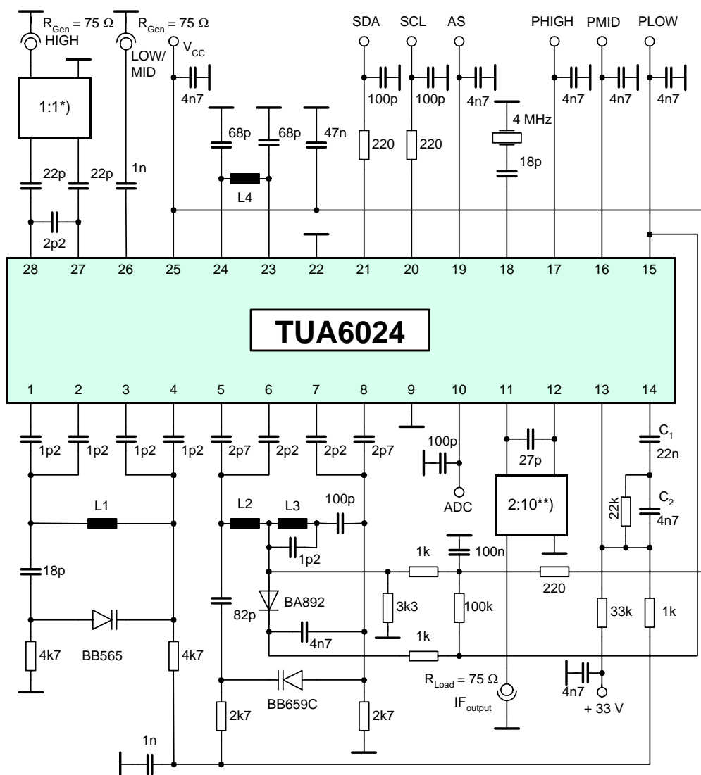
Figure 4-1 Evaluation Board
