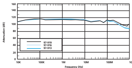
SOLID TOP S 3 TRANSFER IMPEDANCE
