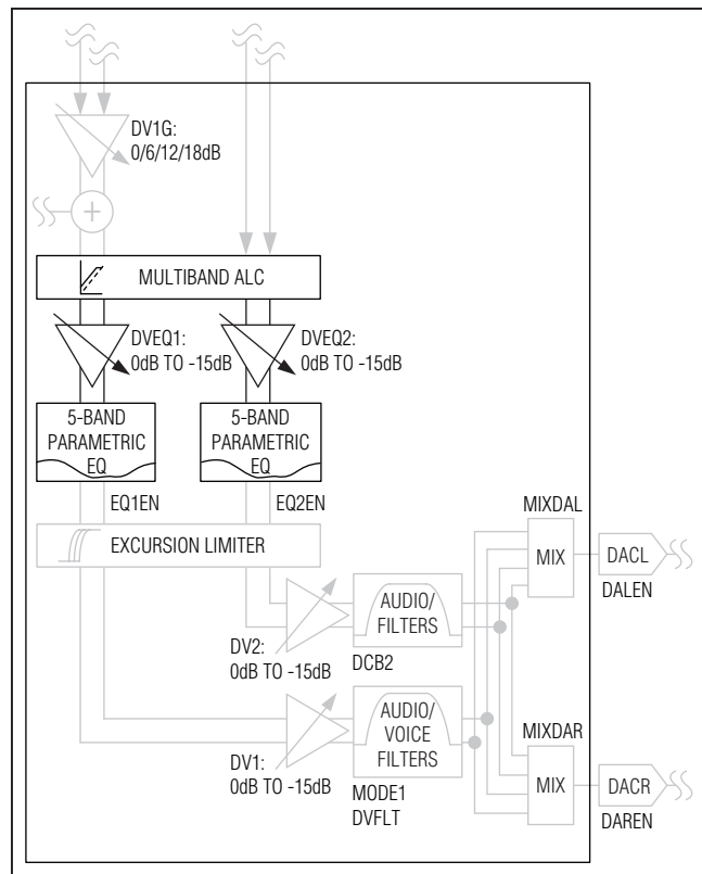
Figure 19. Playback Path Signal Processing Block Diagram
