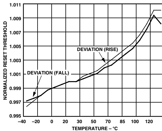
TPC 4. Normalized Reset Threshold vs. Temperature
