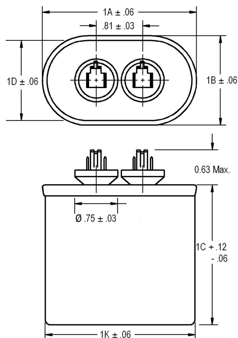
Oval Case Style (A, B, C, D)
