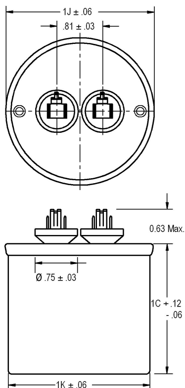
Round Case Style (P, S, T)
