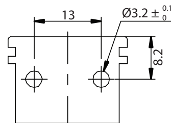
PANEL CUTOUT
