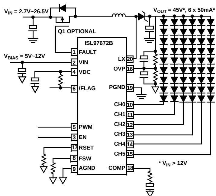
FIGURE 24. DUAL SUPPLY 2.7V OPERATION
