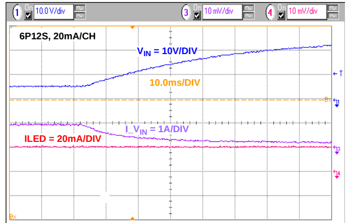
FIGURE 15. LINE REGULATION WITH V_{IN} CHANGE FROM 6V TO 26V, 6P12S AT 20mA/CHANNEL
