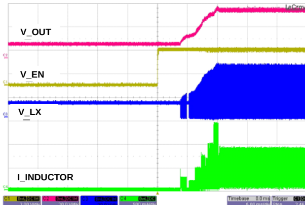
FIGURE 14. STARTUP WAVEFORMS AT V_{IN} = 12V FOR 6P12S AT 20mA/CHANNEL
