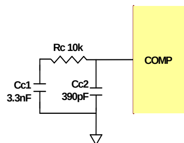
FIGURE 25. COMPENSATION CIRCUIT
