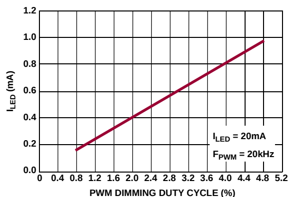
FIGURE 2. DIMMING LINEARITY AT 20kHz
