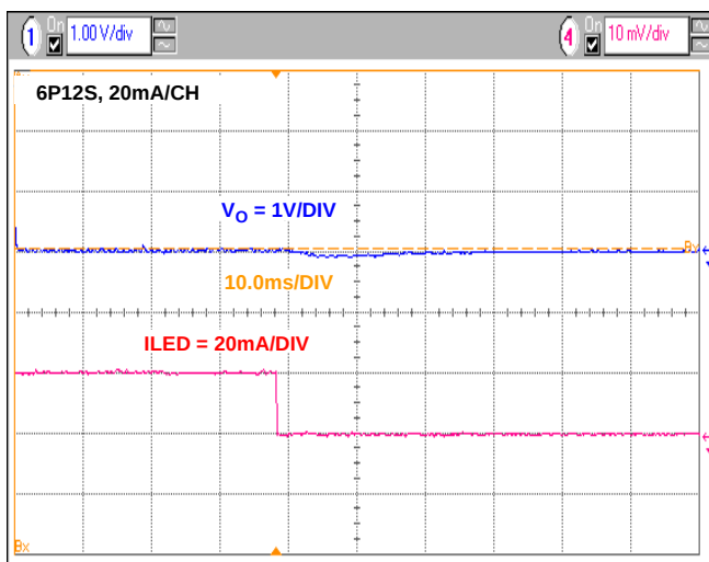
FIGURE 18. BOOST OUTPUT VOLTAGE WITH BRIGHTNESS CHANGE FROM 100% TO 0%, V_{IN} = 12V , 6P12S AT 20mA/CHANNEL
