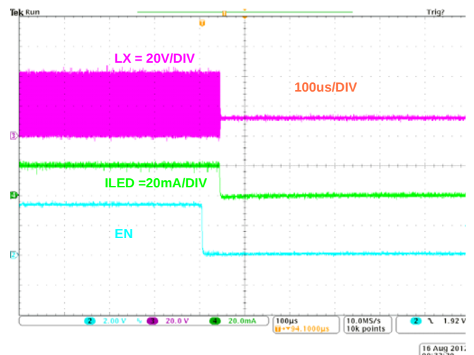
FIGURE 19. ISL97672B SHUTS DOWN AND STOPS SWITCHING ~30 \mu s AFTER EN GOES LOW
