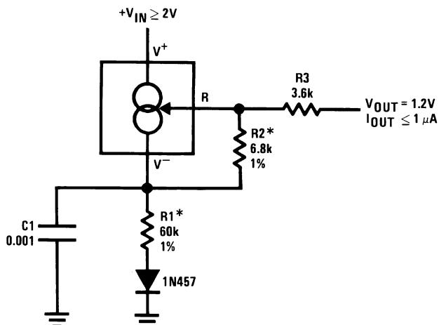
Figure 25. 1.2V Reference Operates on 10 μA and 2V
