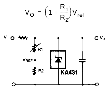
Figure 11. Shunt Regulator
