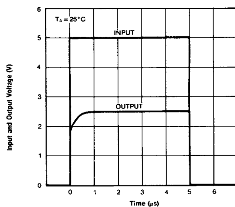
Figure 9. Pulse Response
