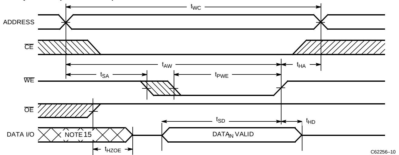
Write Cycle No. 1 ( \overline{WE} Controlled) [8,13,14]
