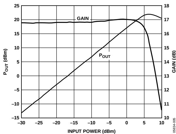
Figure 5. Output Power and Gain vs. Input Power, f = 190\text{ MHz} , V_{POS} = 5\text{ V}
