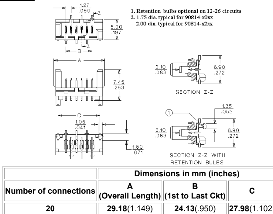
Figure 1. Picoflex Connector
