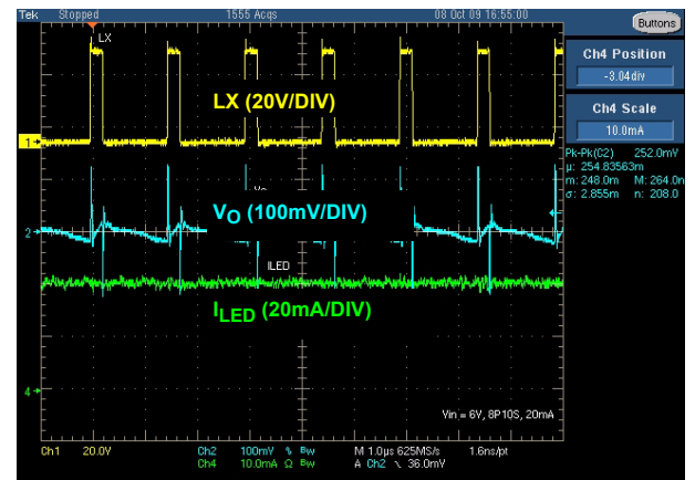
FIGURE 15. V_{OUT} RIPPLE VOLTAGE
