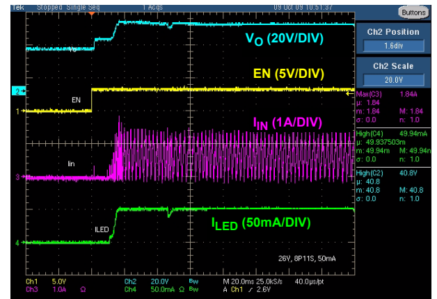
FIGURE 17. IN-RUSH CURRENT and LED CURRENT AT V_{IN} = 26V
