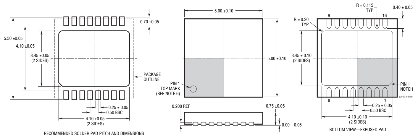
DH Package 16-Lead Plastic DFN (5mm × 5mm) (Reference LTC DWG # 05-08-1709)
