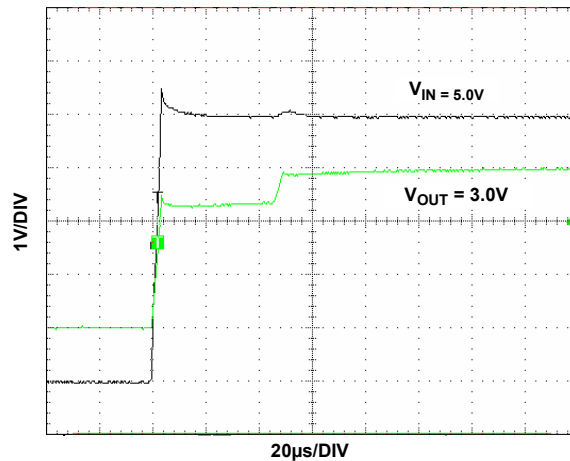
FIGURE 51. TURN-ON TIME
