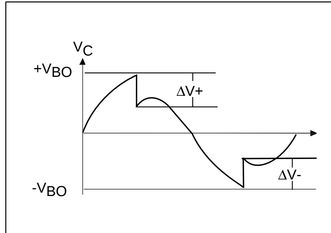
Figure 3.3 Test Circuit Waveforms
