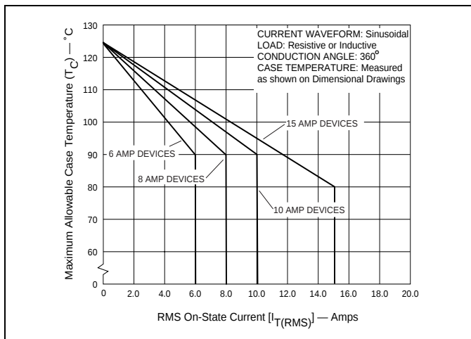
Figure 3.8 Maximum Allowable Case Temperature vs On-State Current (6-15 Amp)
