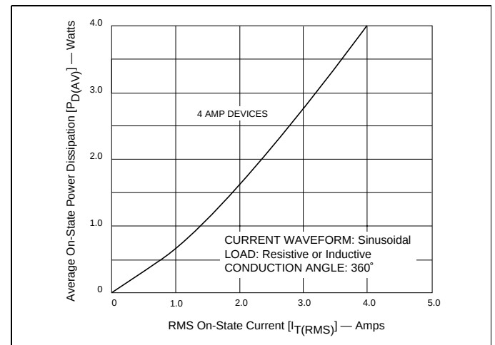
Figure 3.10 Power dissipation (Typical) vs On-State Current (4 Amp)
