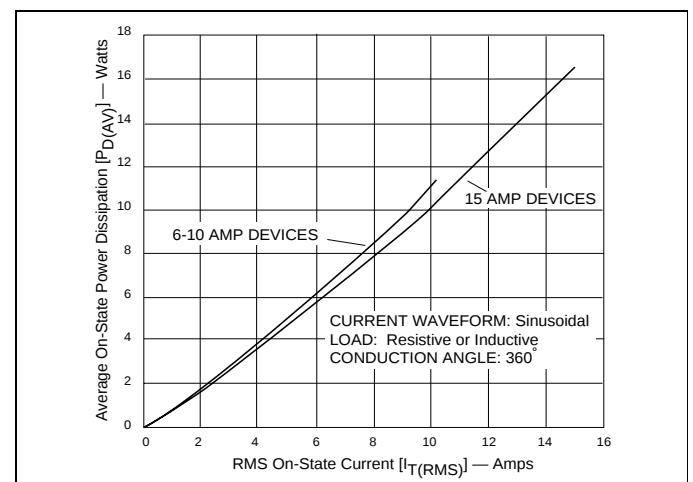
Figure 3.11 Power Dissipation (Typical) vs On-State Current (6-10 and 15 Amp)
