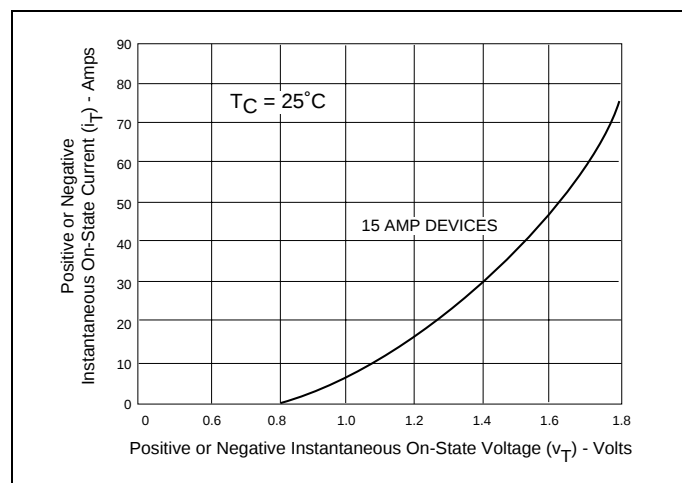
Figure 3.5 On-State Current vs On-State Voltage (Typical) (15 Amp)
