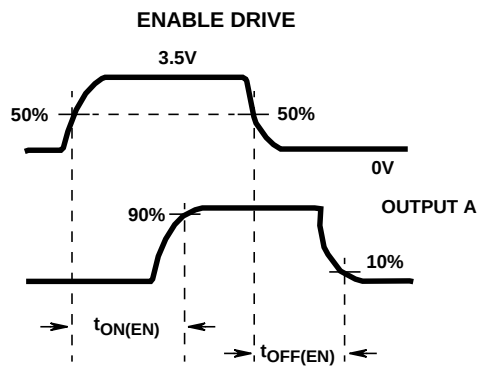
FIGURE 10B. WAVEFORMS
