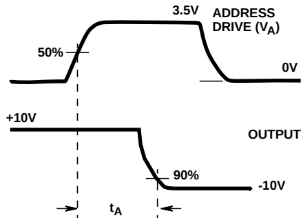
FIGURE 8C. WAVEFORMS
