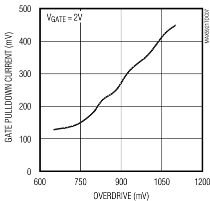
GATE PULLDOWN CURRENT vs. OVERDRIVE DURING A SHORT CIRCUIT
