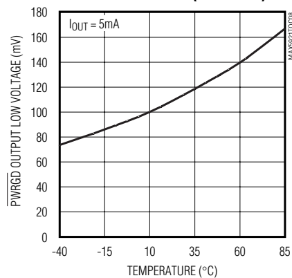
PWRGD OUTPUT LOW VOLTAGE vs. TEMPERATURE (MAX5921A)
