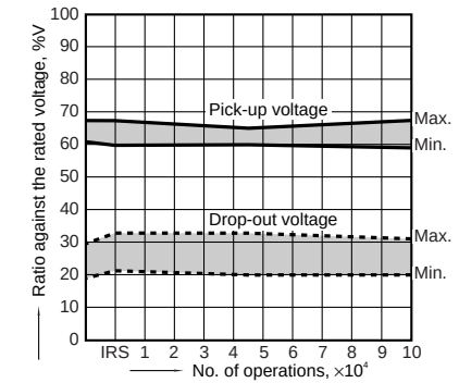
4.-(2) Electrical life (0.5 A 125 V AC resistive load) Tested sample: TQ2SA-12V, 6 pcs Operating frequency: 20 cpm Change of pick-up and drop-out voltage (mounting by IRS method)
