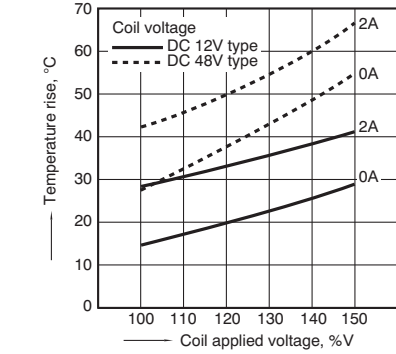
5. Coil temperature rise Tested sample: TQ2SA-12V, 6 pcs. Point measured: Inside the coil Ambient temperature: 25°C 77°F
