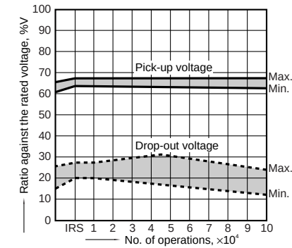
4.-(1) Electrical life (2 A 30 V DC resistive load) Tested sample: TQ2SA-12V, 6 pcs. Operating frequency: 20 cpm Change of pick-up and drop-out voltage (mounting by IRS method)
