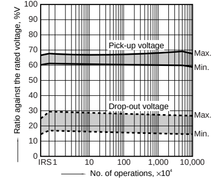
3. Mechanical life (mounting by IRS method) Tested sample: TQ2SA-12V, 10 pcs.
