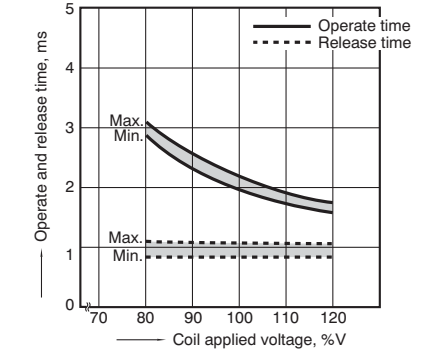
6. Operate/release time Tested sample: TQ2SA-12V, 6 pcs.
