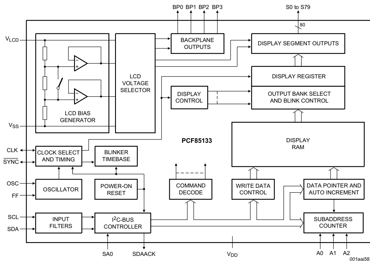
Fig 1. Block diagram of PCF85133
