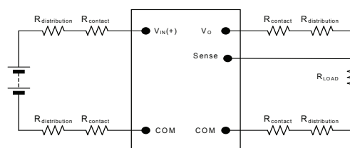
Figure 31. Remote sense circuit configuration
