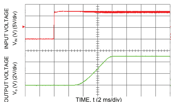
Figure 16. Typical Start-Up with application of V_{in} with low-ESR polymer capacitors at the output ( 7 \times 150\text{ }\mu\text{F} ) ( V_{in} = 12\text{Vdc} , V_o = 5.0\text{Vdc} , I_o = 10\text{A} , C_o = 1050\text{ }\mu\text{F} ).
