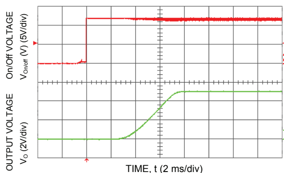
Figure 15. Typical Start-Up Using Remote On/Off with Low-ESR external capacitors ( C_o = 5000\text{ }\mu\text{F} ) ( V_{in} = 12.0\text{Vdc} , V_o = 5.0\text{Vdc} , I_o = 10.0\text{A} , C_o = 1050\text{ }\mu\text{F} ).
