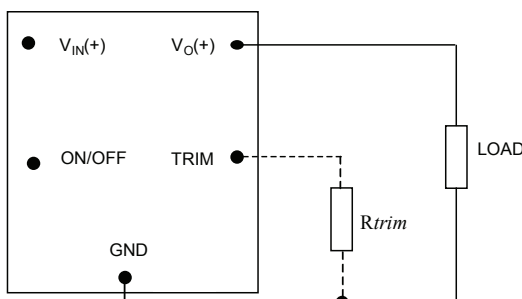
Figure 29. Circuit configuration for programming output voltage using an external resistor.
