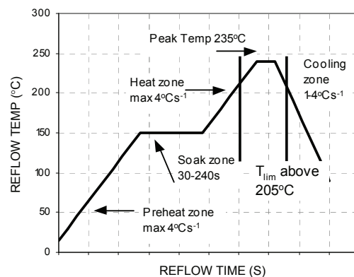
Figure 35. Reflow Profile for Tin/Lead (Sn/Pb) process.
