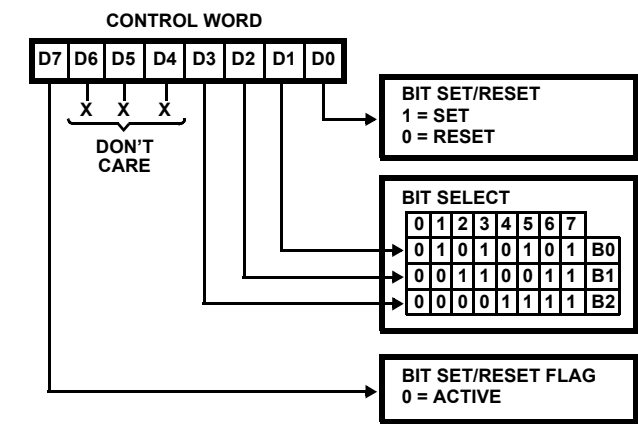
FIGURE 5. BIT SET/RESET FORMAT
