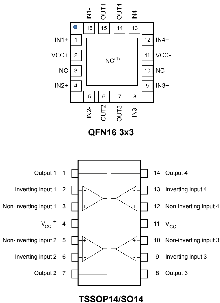
Figure 1. Pin connections (top view)
