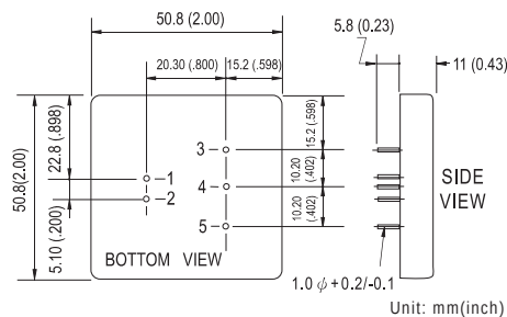
▲ DKE15 2" x 2" x 0.43"
