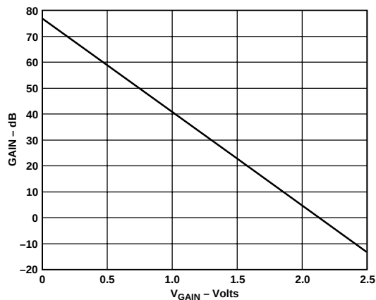
Figure 22. System (Mixer + IF Ceramic Filter + IF Amplifier + Demodulator) Conversion Gain vs. V_{GAIN} , T_A = +25^\circ\text{C} , V_{POS} = 3.0\text{ V} , F_{IF} = 13\text{ MHz} , F_{RF} = 83\text{ MHz} , V_{REF} = 1.2\text{ V}
