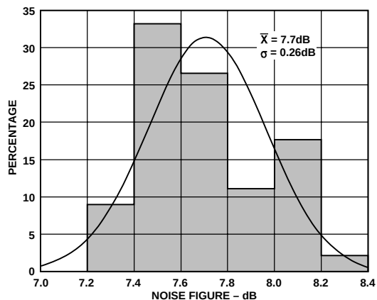
Figure 6. Mixer Noise Figure Histogram, R_S = 1\text{ k}\Omega , F_{RF} = 83\text{ MHz} , F_{IF} = 13\text{ MHz}
