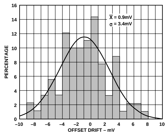
Figure 26. Demodulation Output Offset Voltage Variation Histogram with Variation Referred to Offset at V_{\text{GAIN}} = 1.2 \text{ V} and T_A = +25^\circ\text{C} , V_{\text{GAIN}} = 0.2 \text{ V} and T_A = -25^\circ\text{C}
