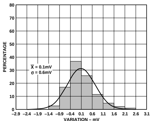
Figure 24. Demodulation Output Offset Voltage Variation Histogram with Variation Referred to Offset at V_{\text{GAIN}} = 1.2 \text{ V} and T_A = +25^\circ\text{C} , V_{\text{GAIN}} = 0.5 \text{ V} and T_A = +25^\circ\text{C}
