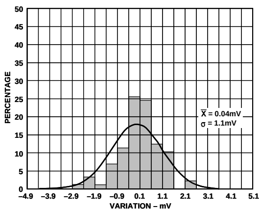
Figure 25. Demodulation Output Offset Voltage Variation Histogram with Variation Referred to Offset at V_{\text{GAIN}} = 1.2 \text{ V} and T_A = +25^\circ\text{C} , V_{\text{GAIN}} = 0.2 \text{ V} and T_A = +25^\circ\text{C}
