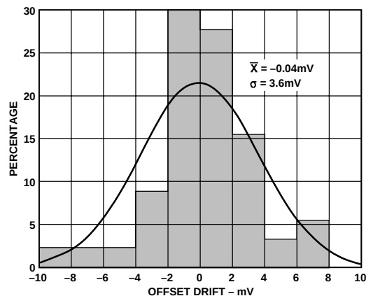
Figure 27. Demodulation Output Offset Voltage Variation Histogram with Variation Referred to Offset at V_{\text{GAIN}} = 1.2 \text{ V} and T_A = +25^\circ\text{C} , V_{\text{GAIN}} = 0.2 \text{ V} and T_A = +85^\circ\text{C}
