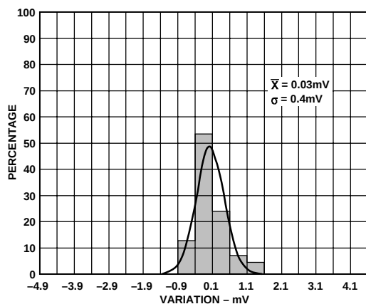
Figure 23. Demodulation Output Offset Voltage Variation Histogram with Variation Referred to Offset at V_{\text{GAIN}} = 1.2 \text{ V} and T_A = +25^\circ\text{C} , V_{\text{GAIN}} = 2.25 \text{ V} and T_A = +25^\circ\text{C}
