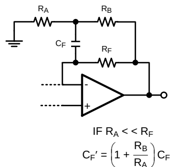
Figure 51. Modified Transimpedance Amplifier
