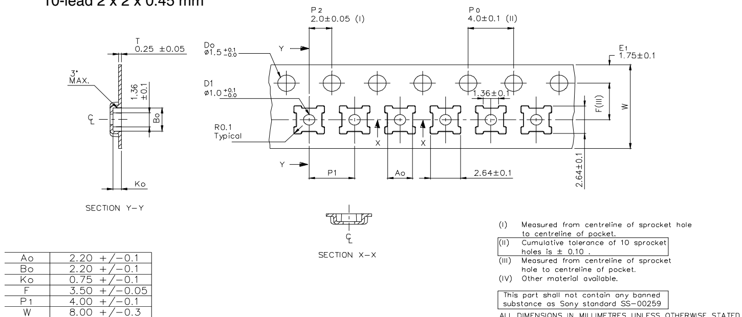
Figure 24. Tape and Reel Specifications
