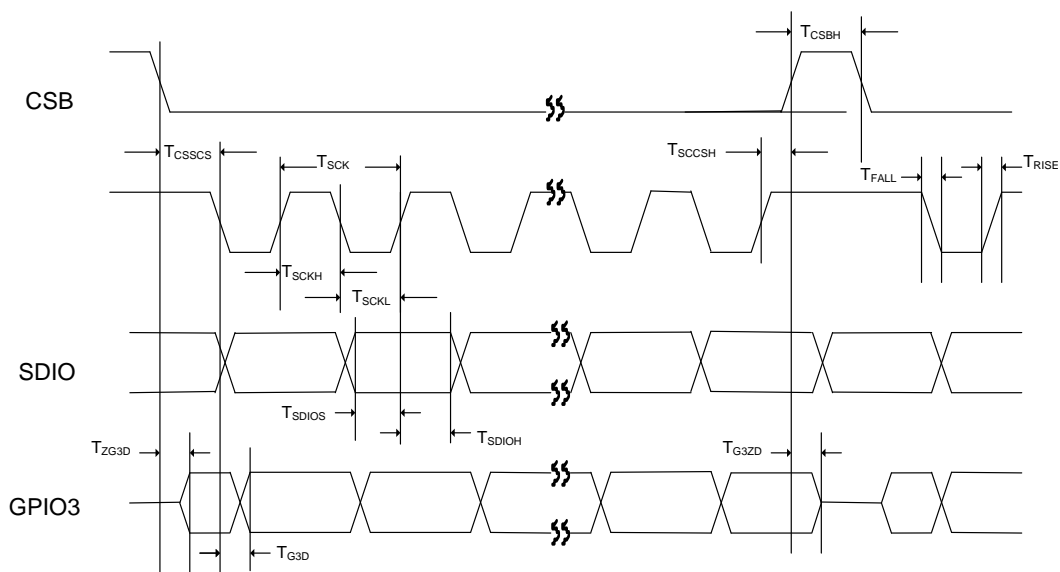
Figure 31: 4-wire ControlMode Timing
