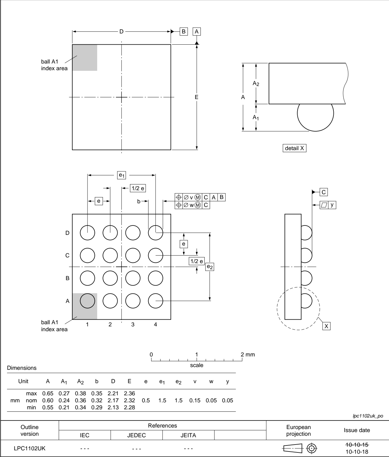
Fig 24. Package outline LPC1102UK (WLCSP16)
