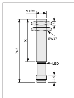
M12 long, screened
