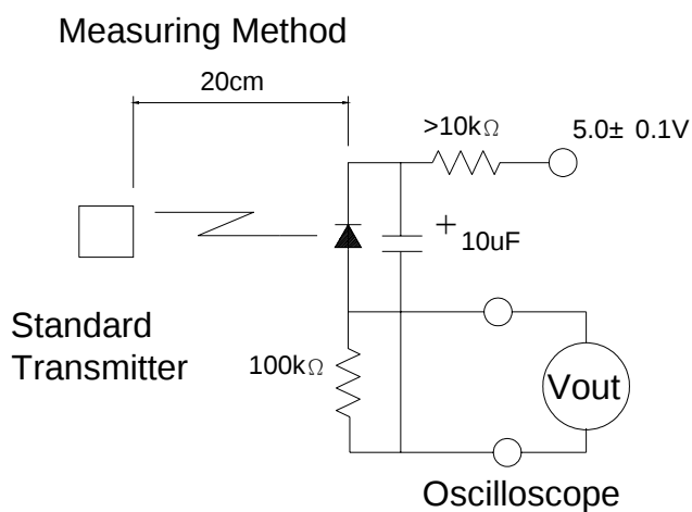
Fig.2 Measuring Method
