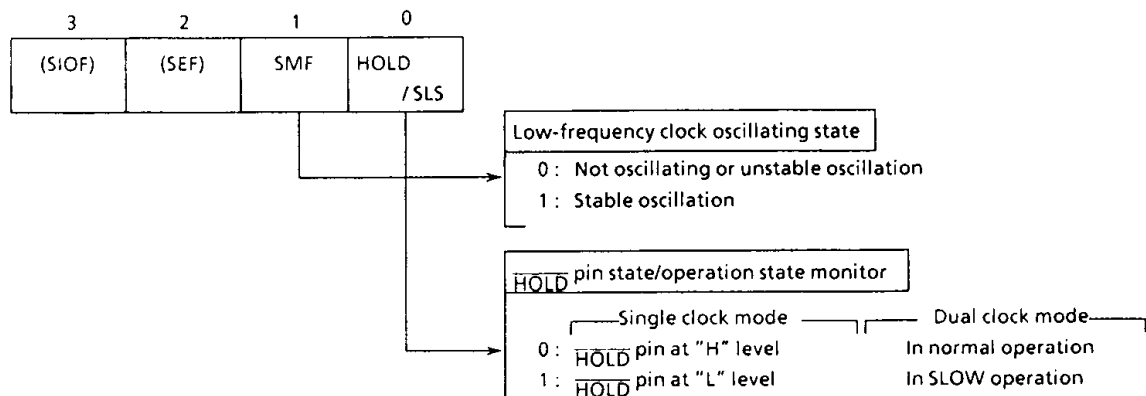
Figure 2-18. System Clock Control Status Register
