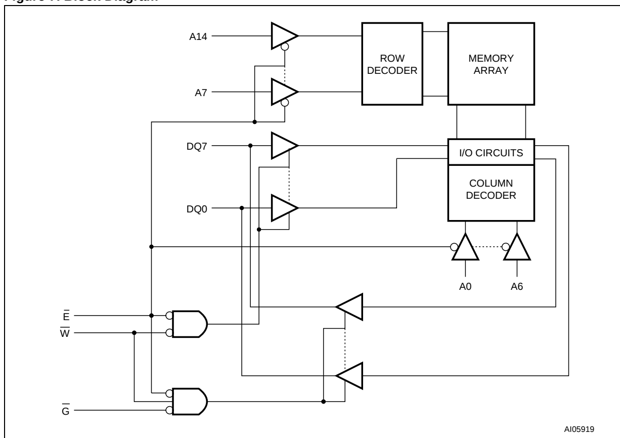
Figure 7. Block Diagram
