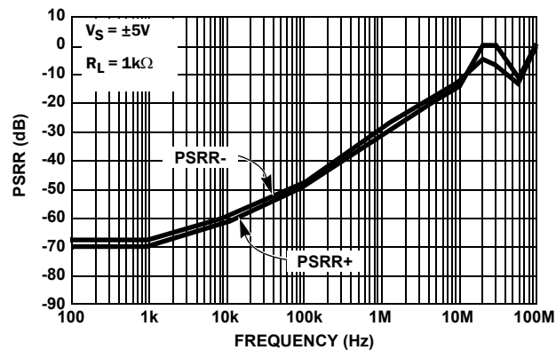
FIGURE 18. PSRR vs FREQUENCY
