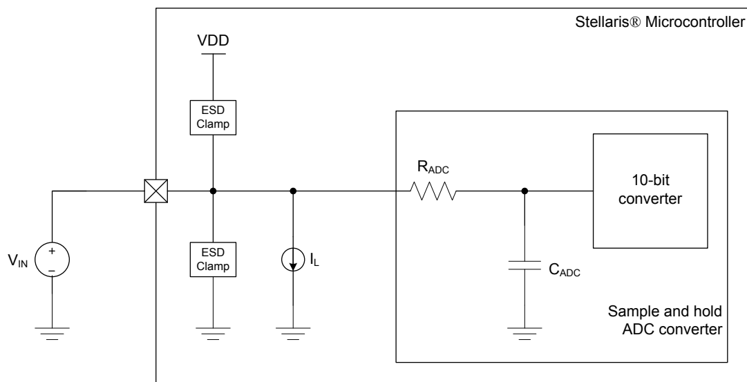
Figure 21-13. ADC Input Equivalency Diagram
