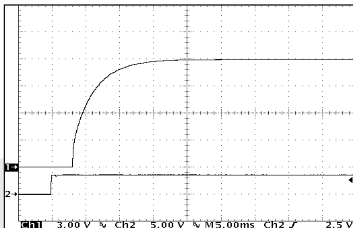
Figure 7: Turn-on transient at full resistive load and zero output capacitance initiated by ENA1. Input voltage pre-applied. Ch 1: Vout (3V/div). Ch 2: ENA1 (5V/div).
