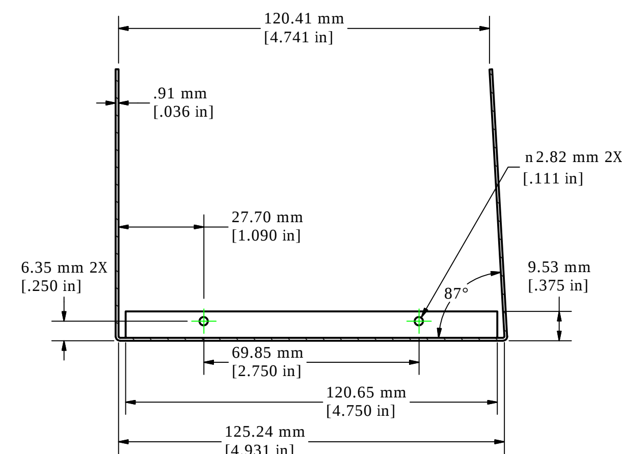
SECTION A-A END VIEW OF EXPLODED ASSEMBLY
