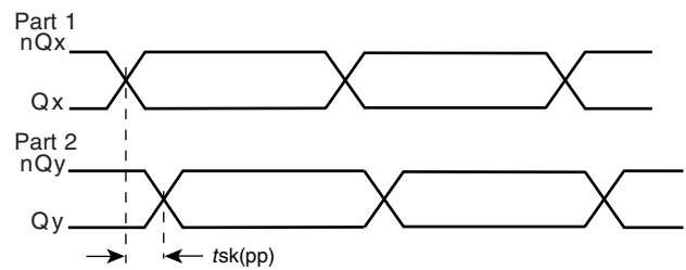
PART-TO-PART SKEW
