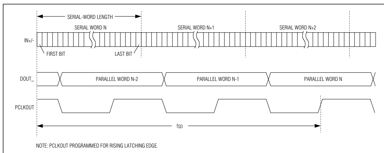
Figure 7. Deserializer Delay
