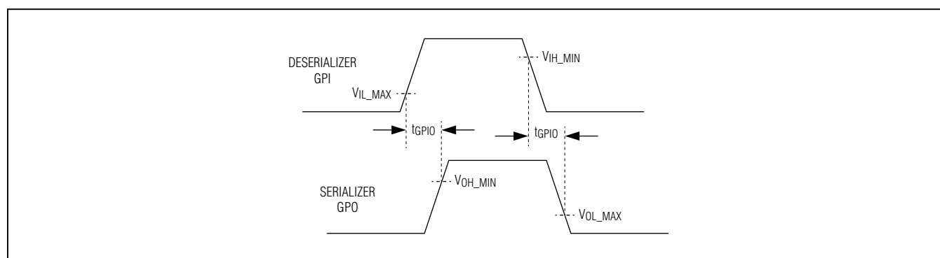
Figure 8. GPI-to-GPO Delay
