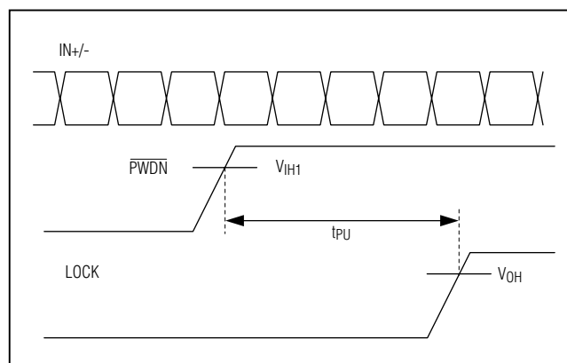
Figure 10. Power-Up Delay
