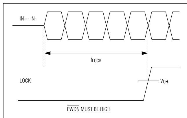
Figure 9. Lock Time
