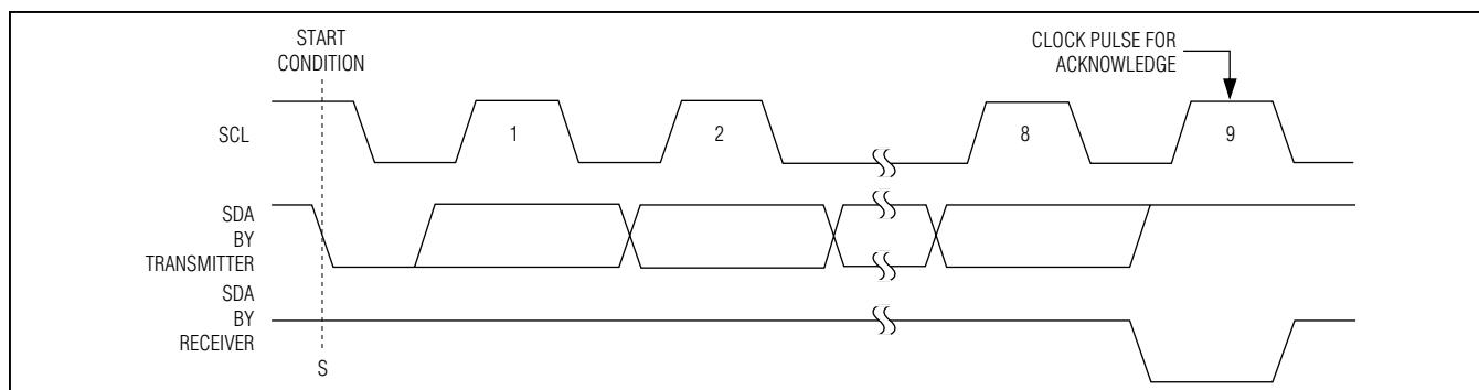
Figure 24. Acknowledge
