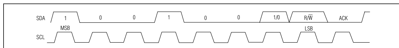
Figure 25. Slave Address
