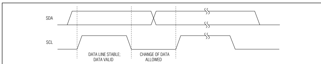
Figure 23. Bit Transfer
