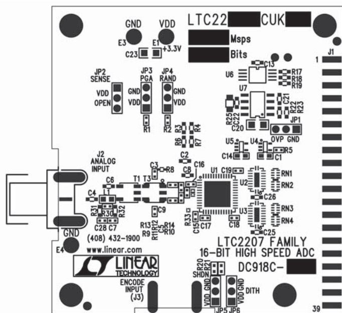
Silkscreen Top
