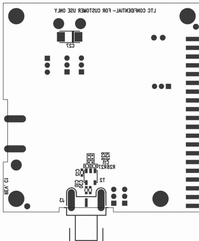
Silkscreen Bottom
