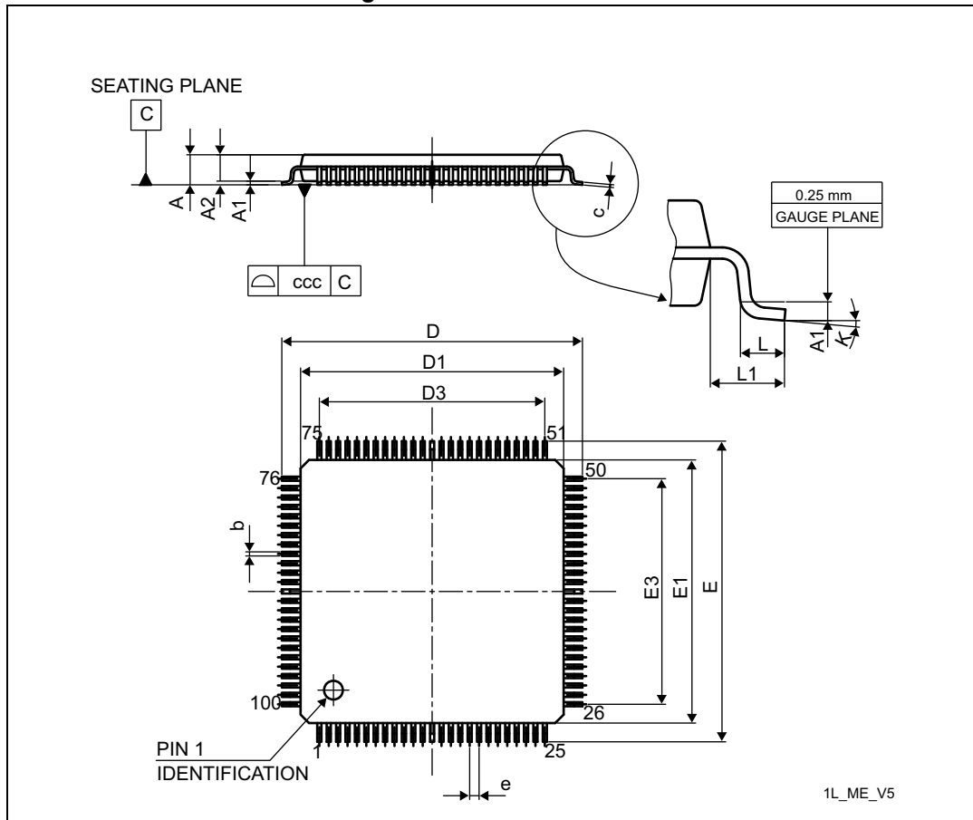
Figure 81. LQFP100 outline
